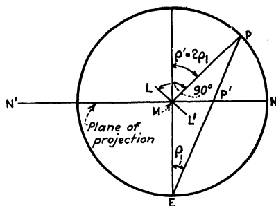
FIG. 9b.—Stereographic projection of the plane LL' .
